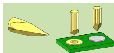
Square lance (33,38,43) For via holes and solder pads. The sharp edges penetrate flux residues and oxide layers.
