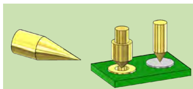
Conical (01,02,03,10,18,32,34,35) Universal tip style with different angles of 10°, 15°, 30°, 60°, 90° or 120° for contacting solder pads and vias.
