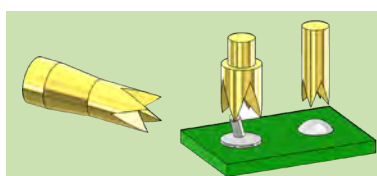
4-point crown (14,20,21,28,29,37) For pad surfaces and soldered pins. The sharp edges penetrate flux residues and oxide layers.
