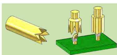
Crown (09,35,40,41,42,60,63) For wire wrap posts, even if the contacts are bent or twisted.
