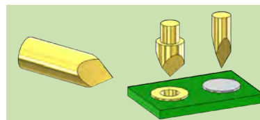
Triangular (15,30,62) For via holes and solder pads. The sharp edges penetrate flux residues and oxide layers.
