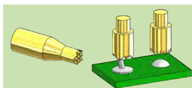
Serrated, W-profile (06,46,64,66) Universal tip style for contacting wires, pins and wire wrap posts, even suitable for bent contacts.
