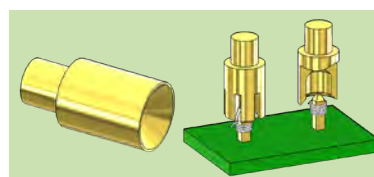
Concave (05,50,55) For a smooth contact of pins and wire wrap posts. The risk of contamination can be minimized by using a self cleaning version.
