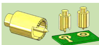
Coaxial design Tip styles of coaxial probes are used for contacting standard connectors or for contacting PCB test points, SMD mini coax and switch connectors, see below.
