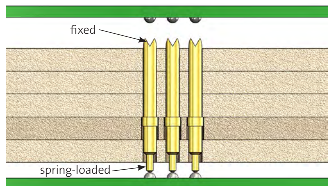
Mounting example FP02
