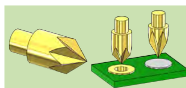
Hexagonal (07,08) For testing plated vias and pads. The sharp edges penetrate contamination and oxide layers.
